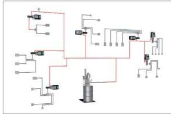
Schematic of a sectional lubrication system with a centralized drum pump and seven EDL1 pressure-booster pumps to supply individual zones
